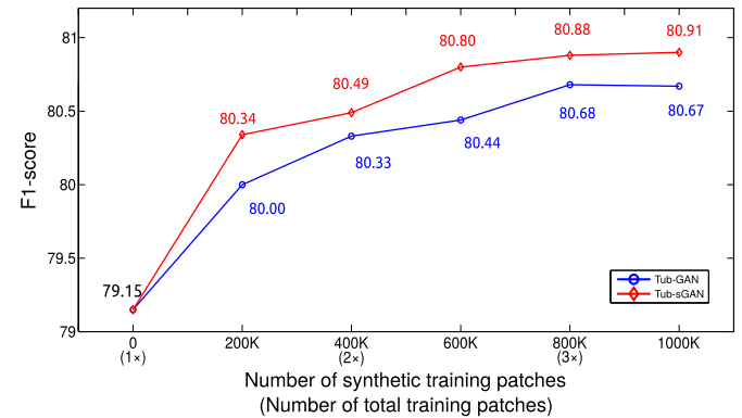
Fig. 13. Performance of our patch-based CNN baseline segmentation method on the DRIVE benchmark as a function of the number of synthetic training patches. The blue and the red curves are the segmentation performances when our Tub-GAN and Tub-sGAN variants are used to synthesize images, respectively. See text for details. (For interpretation of the references to color in this figure legend, the reader is referred to the web version of this article.)
