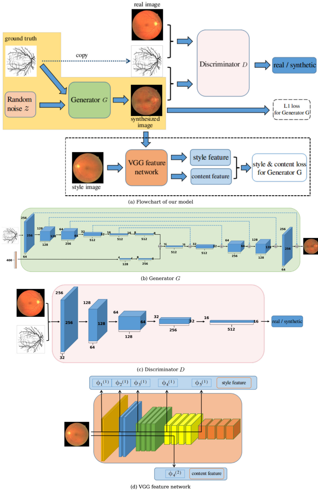
Fig. 1. (a) Flowchart of our approach, which contains the generator and the discriminator networks as detailed in (b) and (c). The dimensions of all layers are specified. The yellow shaded area highlights the generator module that will be engaged in testing. The VGG feature networks are described in (d), where the top row indicates the specific layers (e.g. \phi_1^{(1)}, \phi_2^{(1)}, \dots ) extracted as style features, while the bottom row are the layers (e.g. \phi_4^{(2)} ) used as content features. The \oplus sign denotes a concatenation operation. See text for details.
