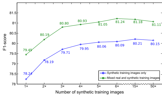
Fig. 14. Performance of our DRIU (Maninis et al., 2016) baseline segmentation model on the DRIVE benchmark as a function of the number of synthetic training images. The blue curve presents results from purely synthetic training images, that is, all images in the training set including the first 20 images are synthesized; The green curve displays results by augmenting the original training set with synthetic images, where the first 20 images are those original training images. See text for details. (For interpretation of the references to color in this figure legend, the reader is referred to the web version of this article.)
